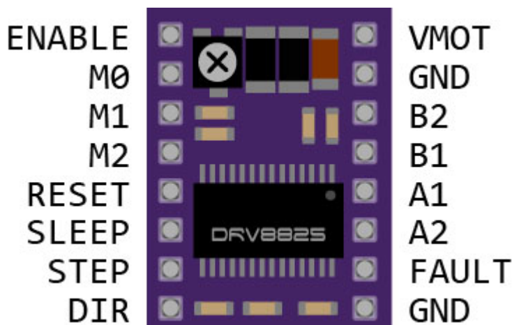
DRV8825 Pinout
